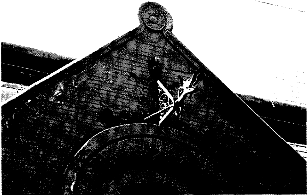
Fire Hook & Ladder Company No. 14 (now Fire Engine Company No. 36) Detail of wrought-iron jib used for hauling hay Photo: Carl Forster
